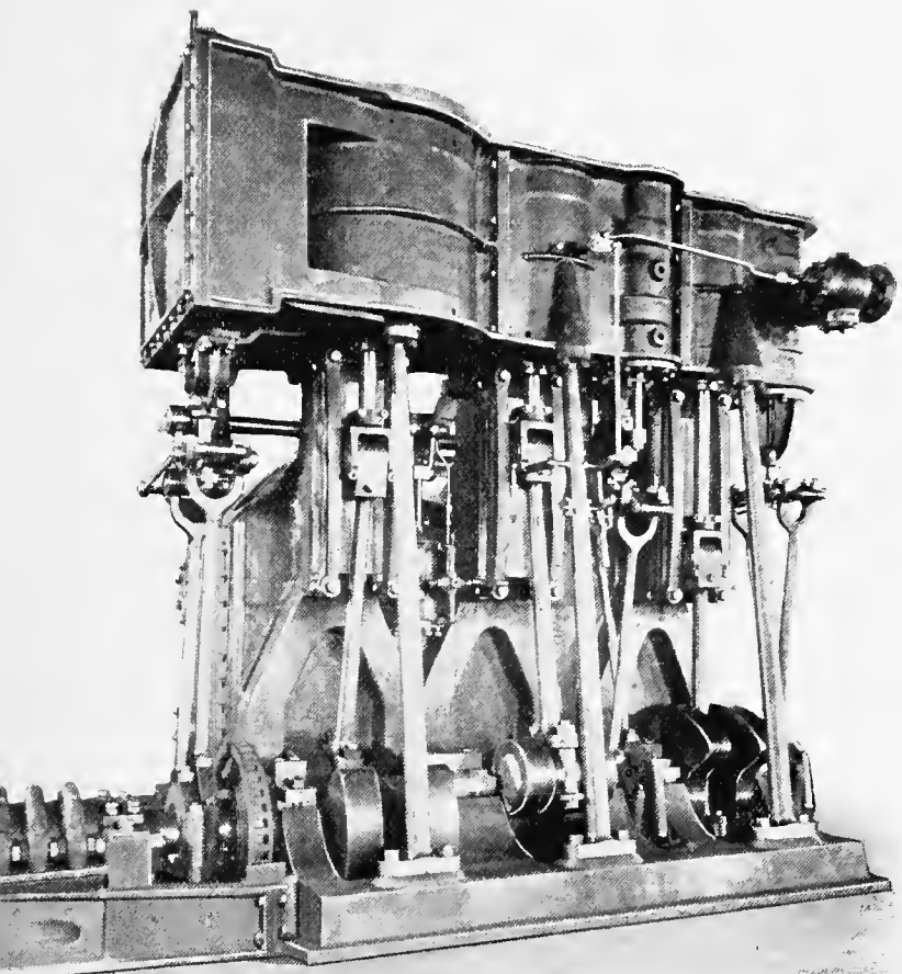
ENGINE OF THE STEAM YACHT FREE LANCE.
